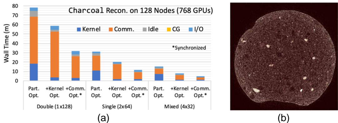
Figure 1. (a) Breakdown of end-to-end reconstruction time for reconstruction of the charcoal dataset on 128 nodes of Summit (on 768 V100 GPUs). (b) A single slice of 3D reconstruction of the charcoal dataset.
